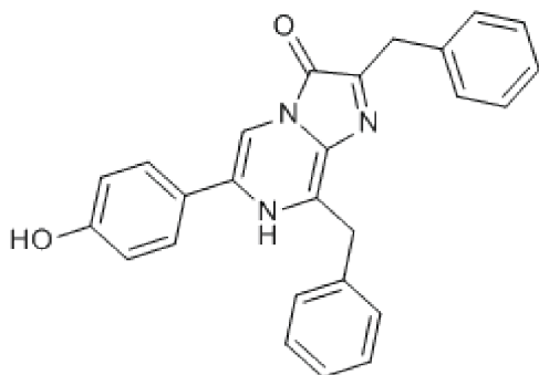
Coelenterazine-h
