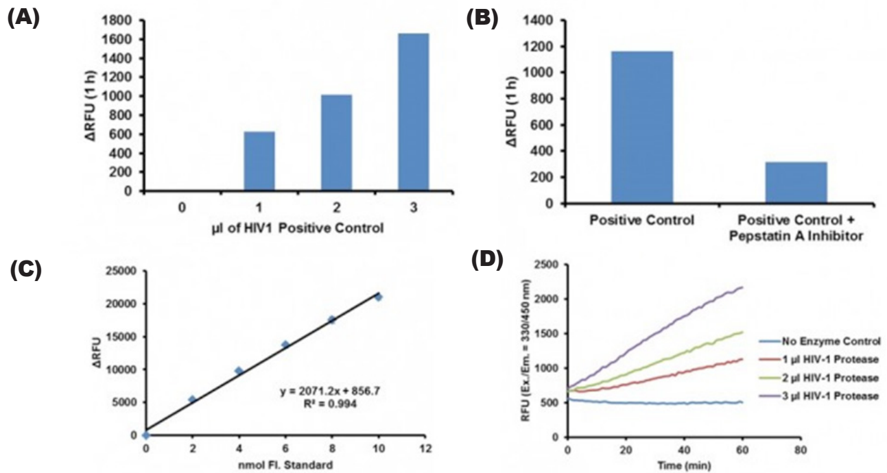
Figure: Measurement of HIV1 Protease activity using HIV-1 Protease as a positive control (A) and its inhibition by Pepstatin A inhibitor (Cat # 1732) (B). FI. Standard plot (C) Progressive activity curves using different amounts of HIV-1 Protease (Positive Control) with time (D). Assays were performed following the K825-100 kit protocol.
